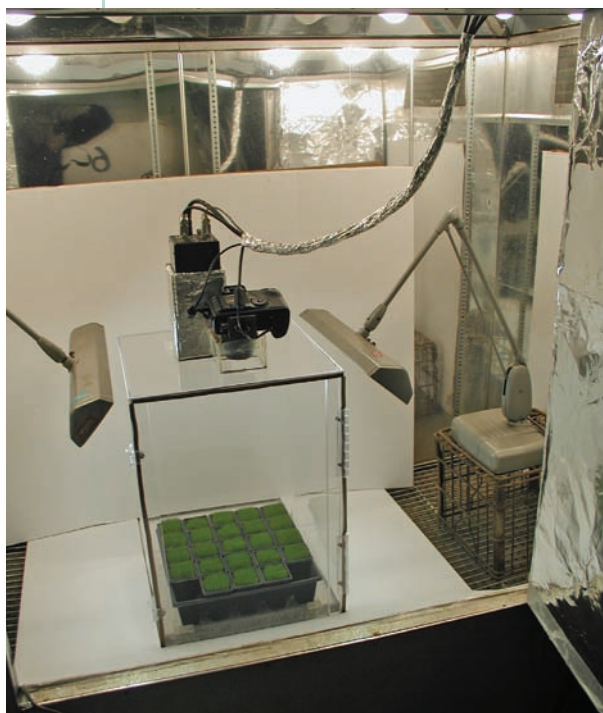
Above: The Plexiglas humidifier is contained in a growth chamber. Image-capturing devices are mounted 15 inches (38 centimeters) above the grass canopies and capture images simultaneously throughout the experiments.
